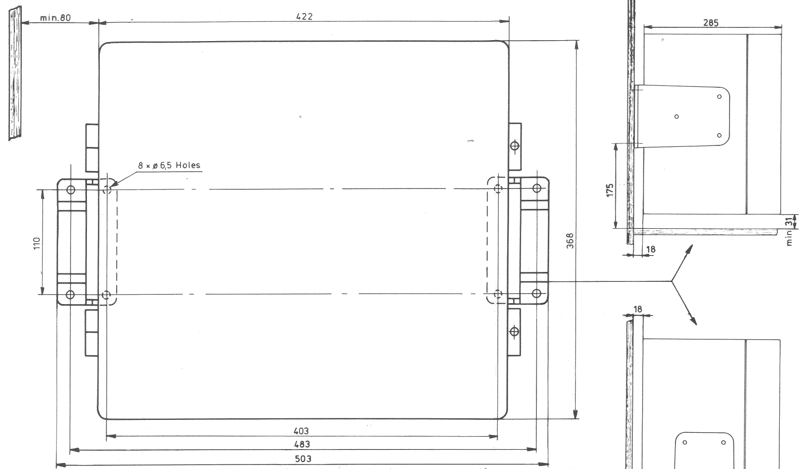
Transceiver Unit
