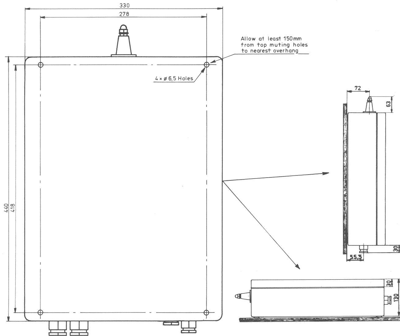
Antenna Tuning Unit
